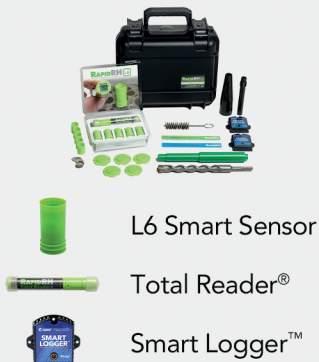
STARTER KIT+ Rapid RH® L6 Concrete Moisture Starter Kit
